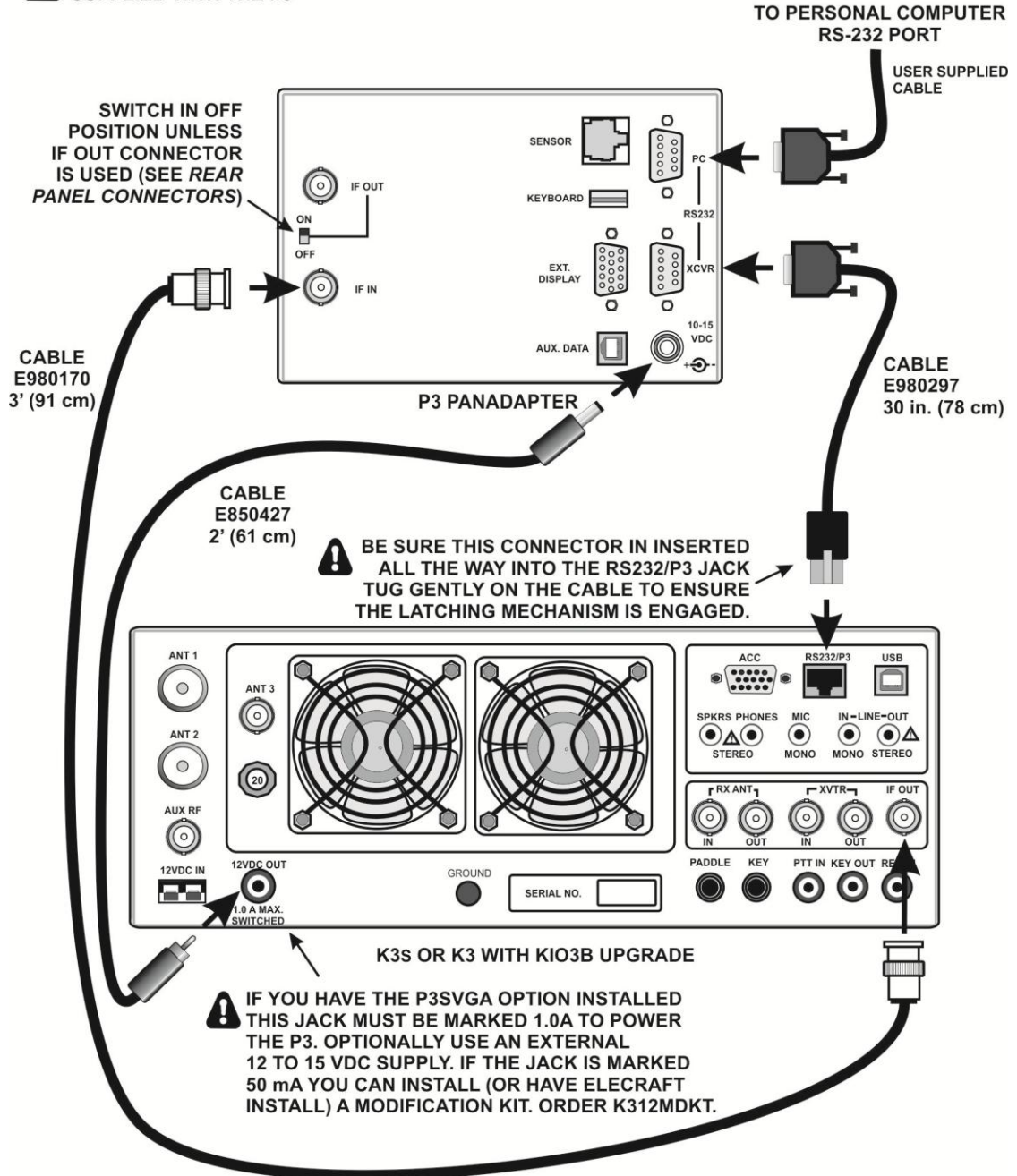
BASIC K3S/P3 CABLING FOR RS-232 INTERFACE TO PERSONAL COMPUTER
