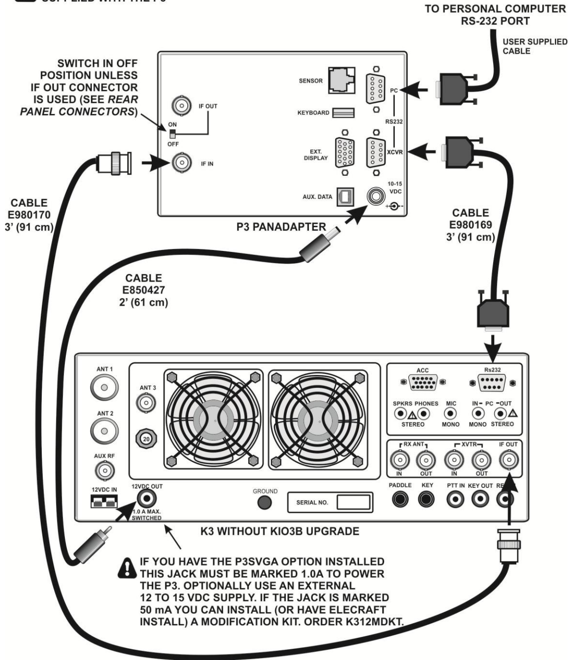
BASIC K3/P3 CABLING FOR RS-232 INTERFACE TO PERSONAL COMPUTER
