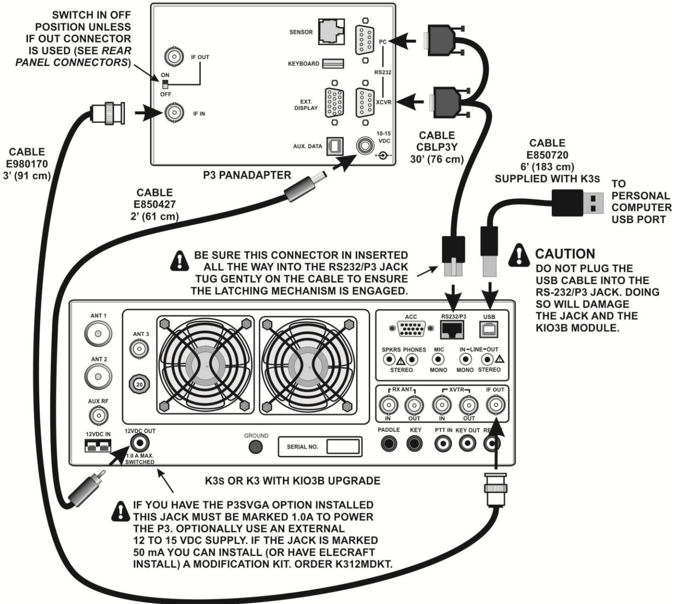
BASIC K3S/P3 CABLING FOR USB INTERFACE TO PERSONAL COMPUTER
